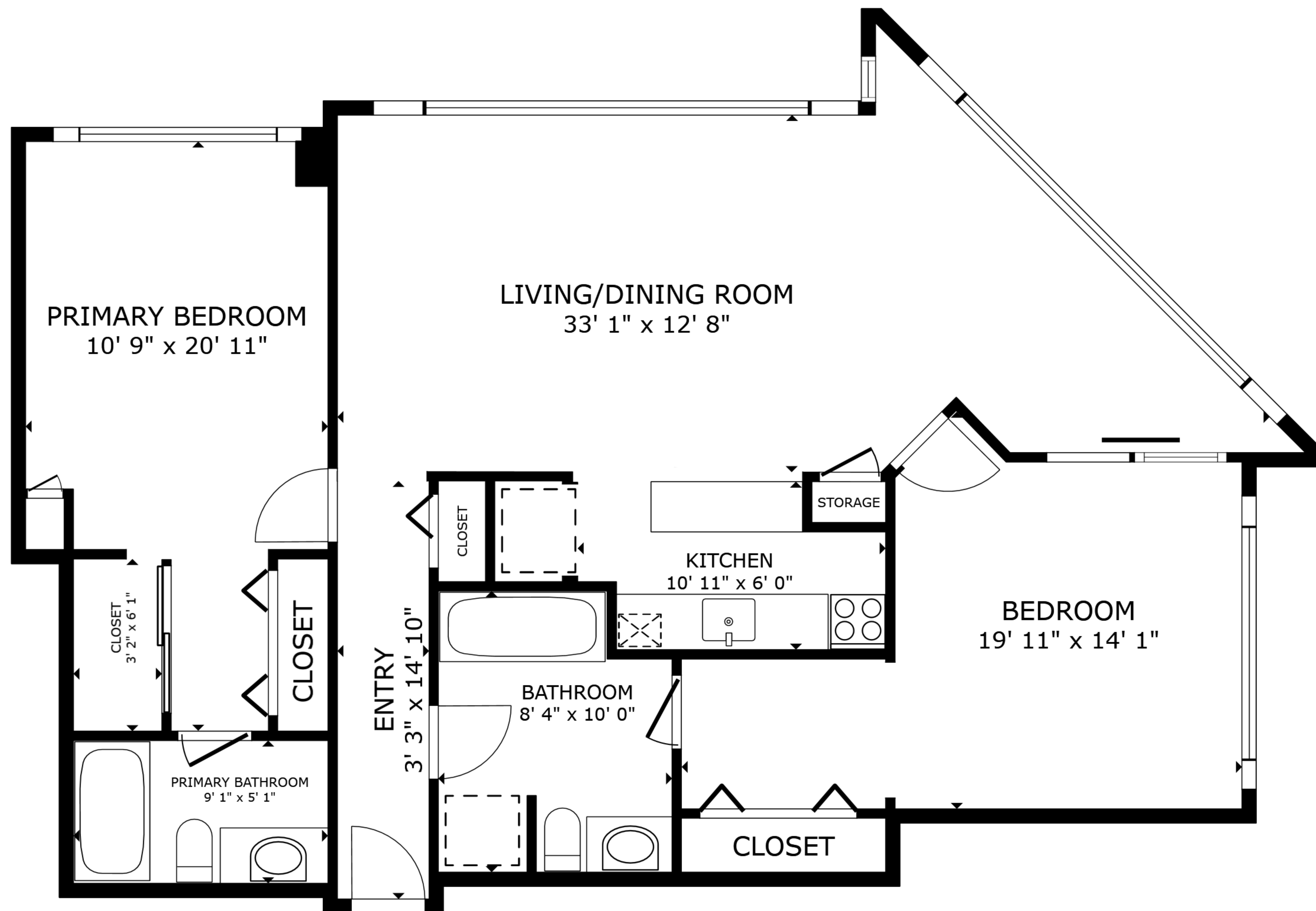
FLOOR PLAN
